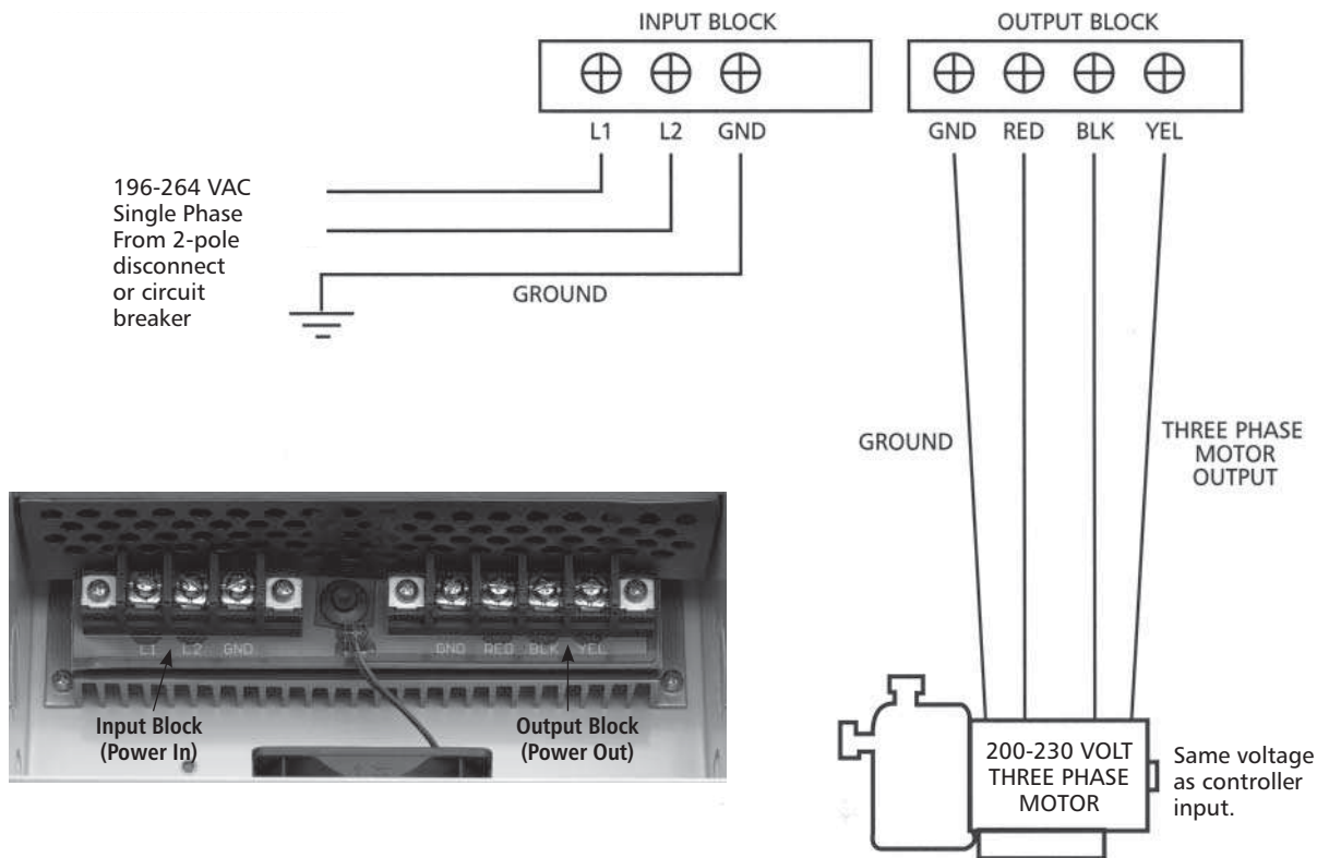
Figure 3 Wiring Diagram
