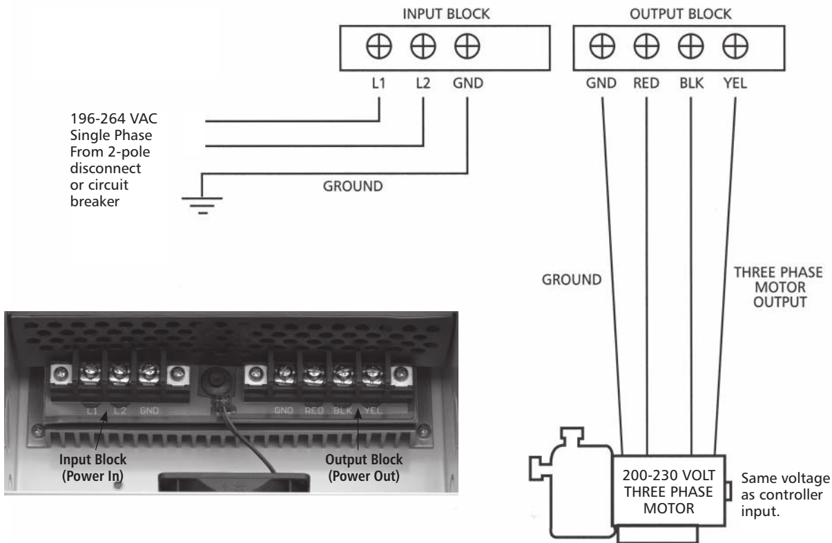
Figure 3 Wiring Diagram
